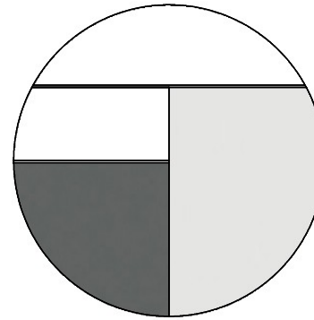
DETAIL C - DOORS OVERLAP THE PILASTERS BY 20mm EITHER SIDE. INWARD DOORS ARE EQUAL HEIGHT TO PILASTERS, OUTWARD DOORS ARE REDUCED BY 50mm IN HEIGHT SO, THEY DO NOT CLASH WITH THE D-SHAPED HEADRAIL.
